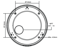
Mounting Plate
